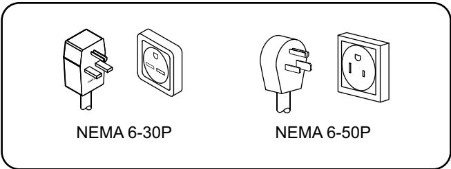
Plug Configuration
